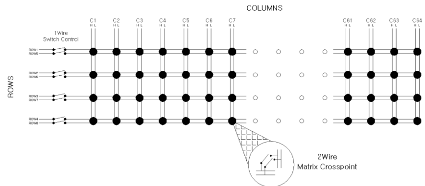
4 X 64 2Switch Matrix channel is shown
